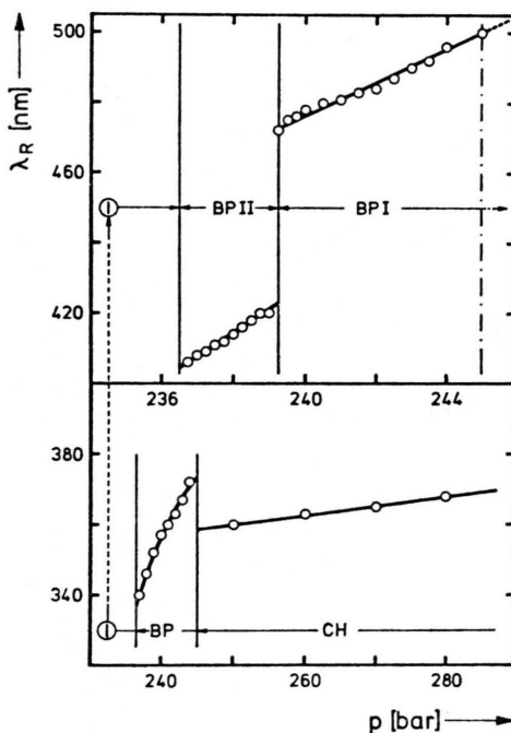
Fig. 1. The pressure ( p ) dependence of the reflection wavelength of maximum light intensity ( \lambda_R ) at constant temperature ( \vartheta = 102^\circ\text{C} ) for cholesteryl nonanoate I = isotropic phase, BP = blue phase, CH = cholesteric phase.
